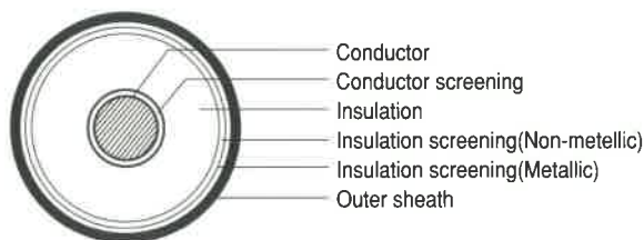
Single core cable
